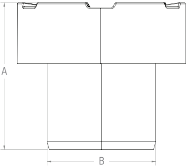
DN90 SURE-VENT ULTRA VALVE
